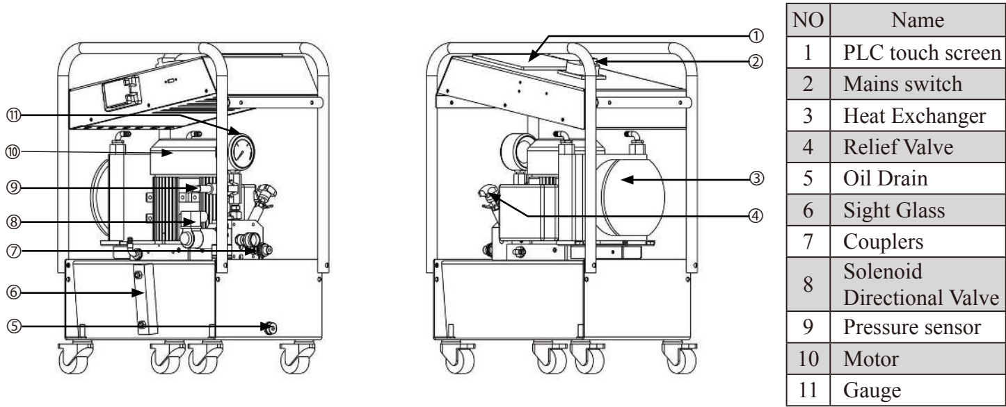
▼ HE5TW10-AT Product Diagram:
