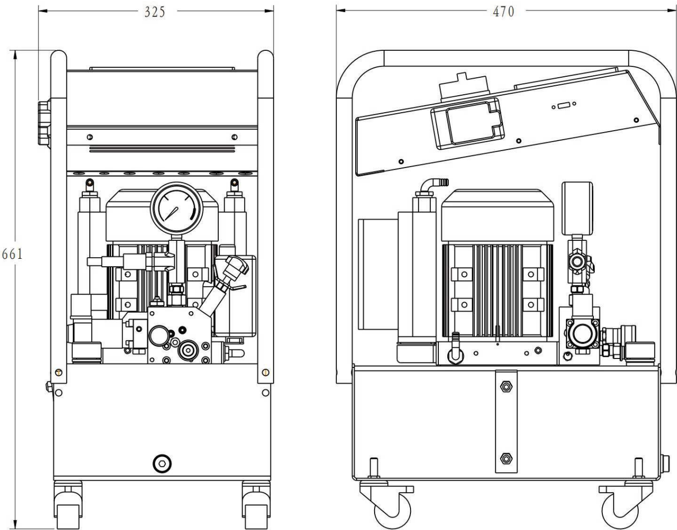
▼ HE5TW10-AT Outline Dimensional Drawing:
