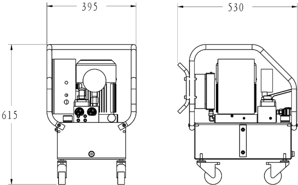
▼ EDP2000-10 Outline Dimensional Drawing:
