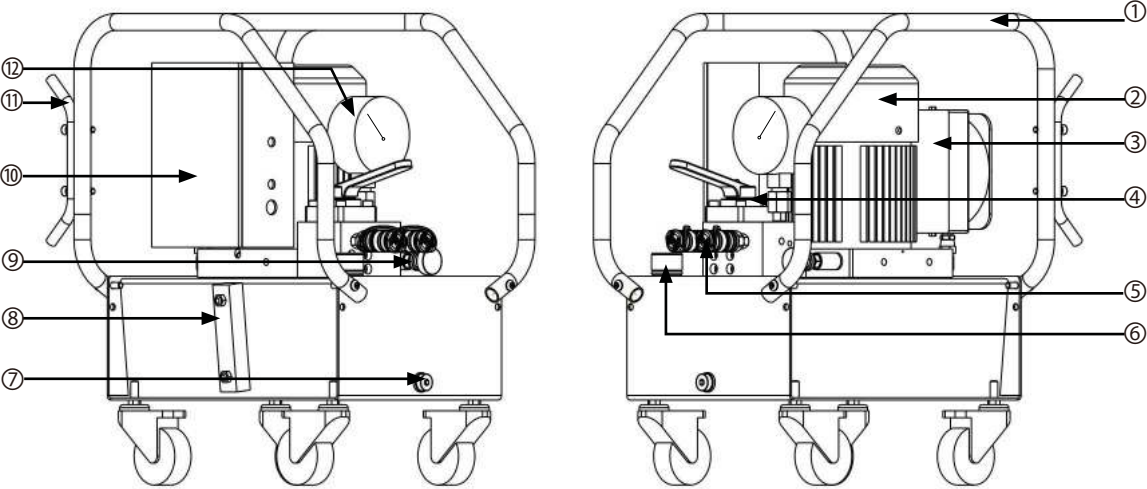
▼ EDP2004-60 Product Illustration :
